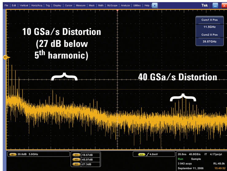
Figure 16b: FFT analysis on a 400-MHz clock using a Tektronix 2.5-GHz bandwidth oscilloscope
