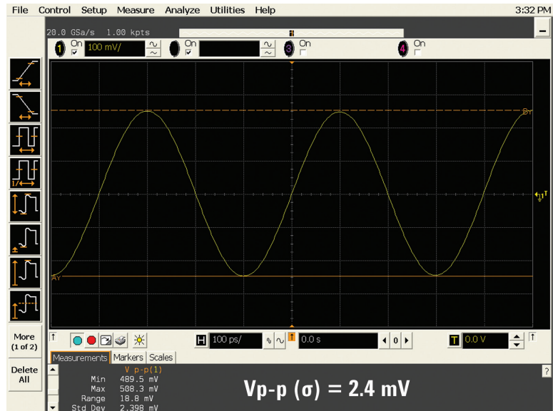
Figure 12a: 2.5-GHz sine wave captured on the Keysight Infiniium oscilloscope sampling at 20 GSa/s (non-interleaved)
