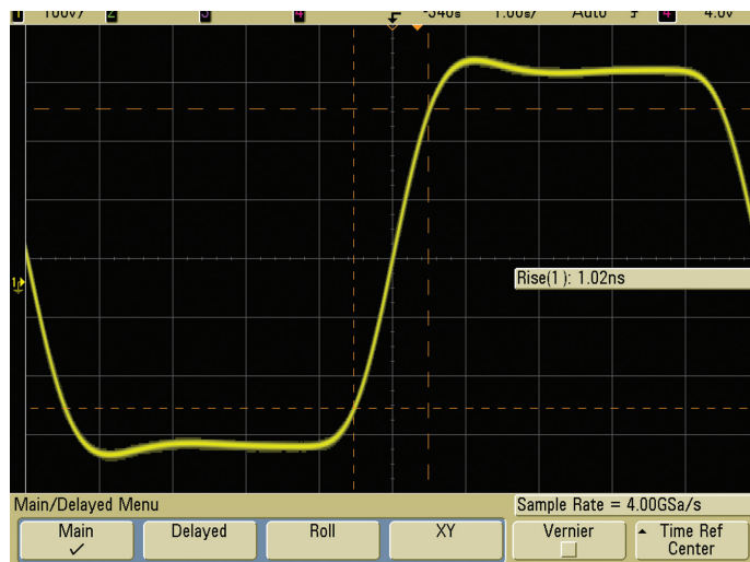
Figure 7: Keysight 500-MHz bandwidth scope sampling at 4 GSa/s produces minimal measurement improvement over sampling at 2 GSa/s
