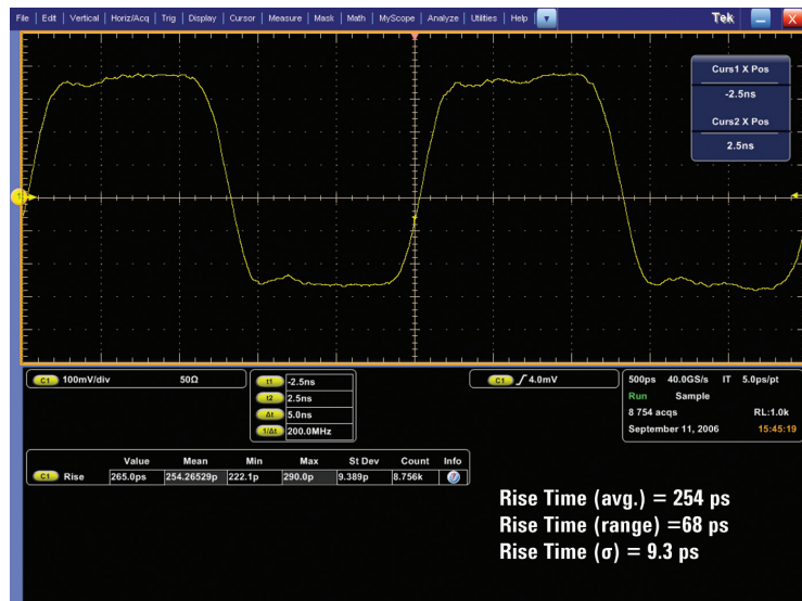
Figure 15b: 400-MHz clock captured on a Tektronix 2.5-GHz oscilloscope sampling at 40 GSa/s
