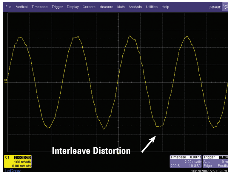
Figure 11b: 200-MHz sine wave captured on a LeCroy 1-GHz bandwidth oscilloscope sampling at 10 GSa/s
