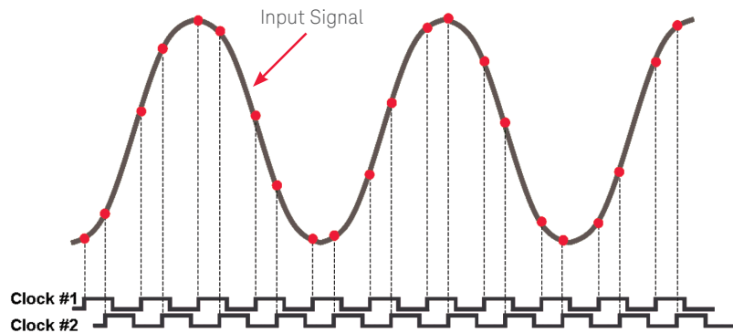
Figure 9: Timing diagram showing non-evenly spaced samples
