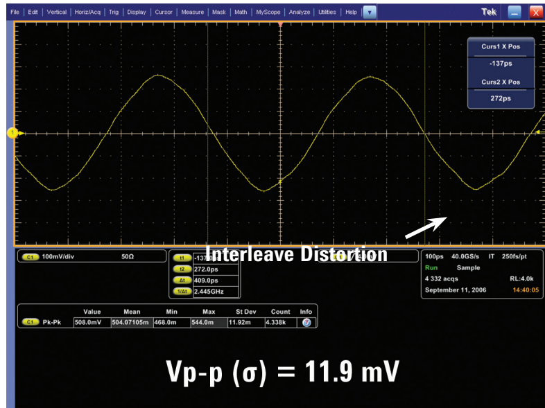
Figure 13b: 2.5-GHz sine wave captured on a Tektronix 2.5-GHz bandwidth oscilloscope sampling at 40 GSa/s (interleaved)
