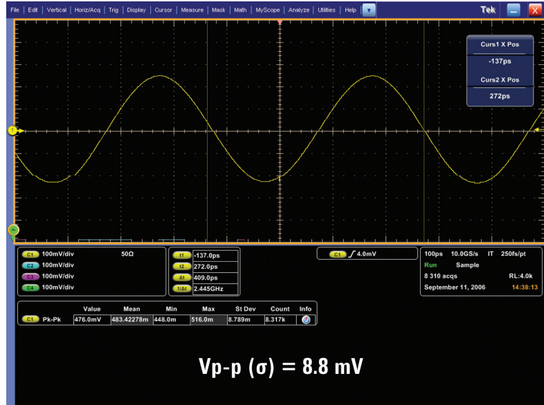
Figure 13a: 2.5-GHz sine wave captured on a Tektronix 2.5-GHz bandwidth oscilloscope sampling at 10 GSa/s (non-interleaved)
