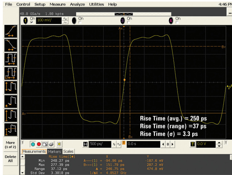
Figure 15a: 400-MHz clock captured on a Keysight Infiniium 3-GHz oscilloscope sampling at 40 GSa/s
