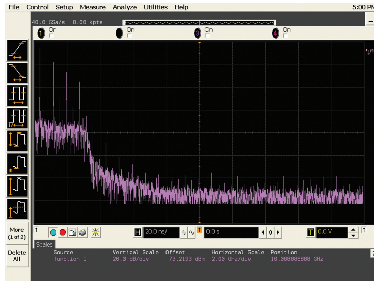
Figure 16a: FFT analysis on a 400-MHz clock using a Keysight Infiniium 3-GHz bandwidth oscilloscope
