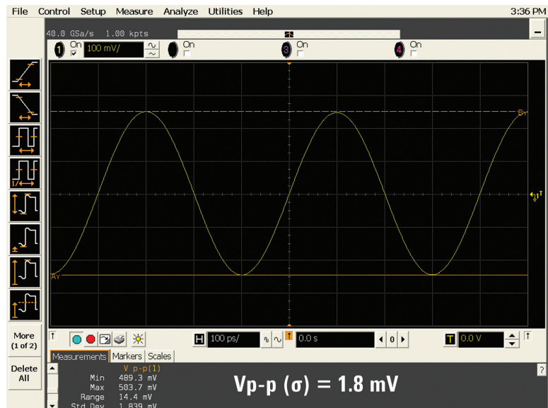
Figure 12b: 2.5-GHz sine wave captured on the Keysight Infiniium oscilloscope sampling at 40 GSa/s (interleaved)
