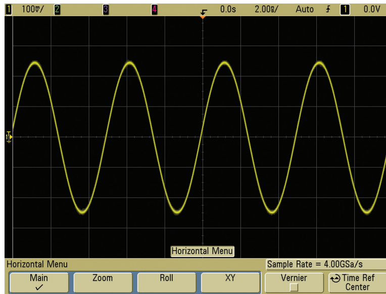
Figure 11a: 200-MHz sine wave captured on a Keysight 1-GHz bandwidth oscilloscope sampling at 4 GSa/s
