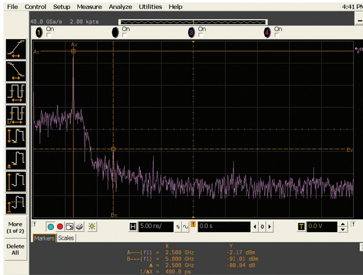
Figure 14a: FFT analysis of 2.5-GHz sine wave captured on a Keysight Infiniium oscilloscope sampling at 40 GSa/s
