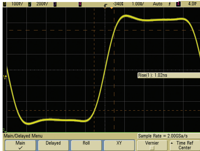
Figure 6: Keysight Technologies, Inc. 500-MHz bandwidth scope sampling at 2 GSa/s shows an accurate measurement of this 100-MHz clock with a 1-ns edge speed
