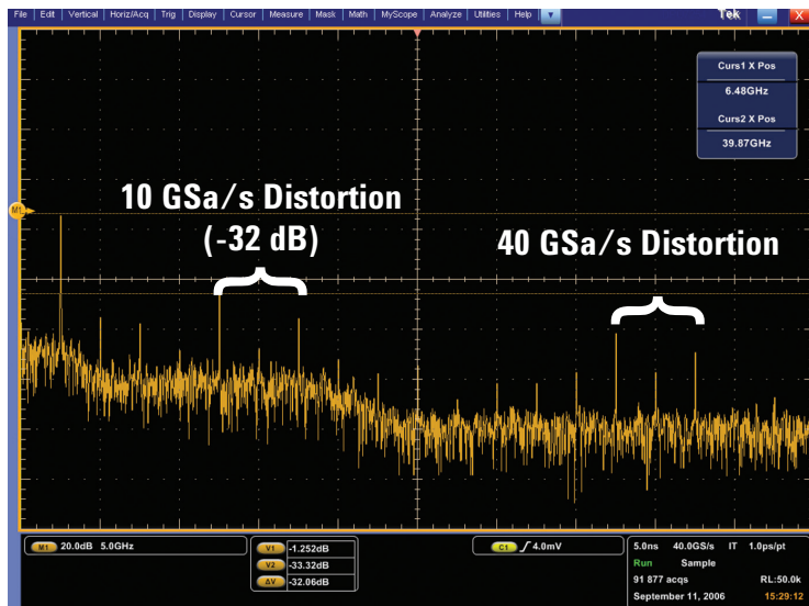
Figure 14b: FFT analysis of 2.5-GHz sine wave captured on a Tektronix oscilloscope sampling at 40 GSa/s
